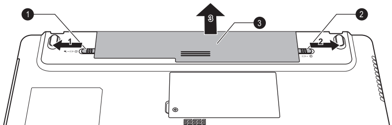
Figure 5-1 Releasing the battery pack (Satellite L770/L775/L770D/L775D/satellite Pro L770/L775/L770D/L775D)
